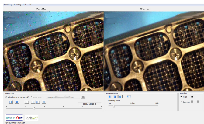
Intuitive SPARKLE Interface
